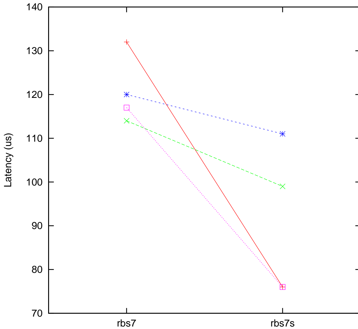
Moderate load maximum latency ARM Freescale i.MX6 Quad 96 MHz, Linux 5.16.2-rt19 vs. ARM Freescale i.MX6 Quad 96 MHz, Linux 5.15.26-xenomai
