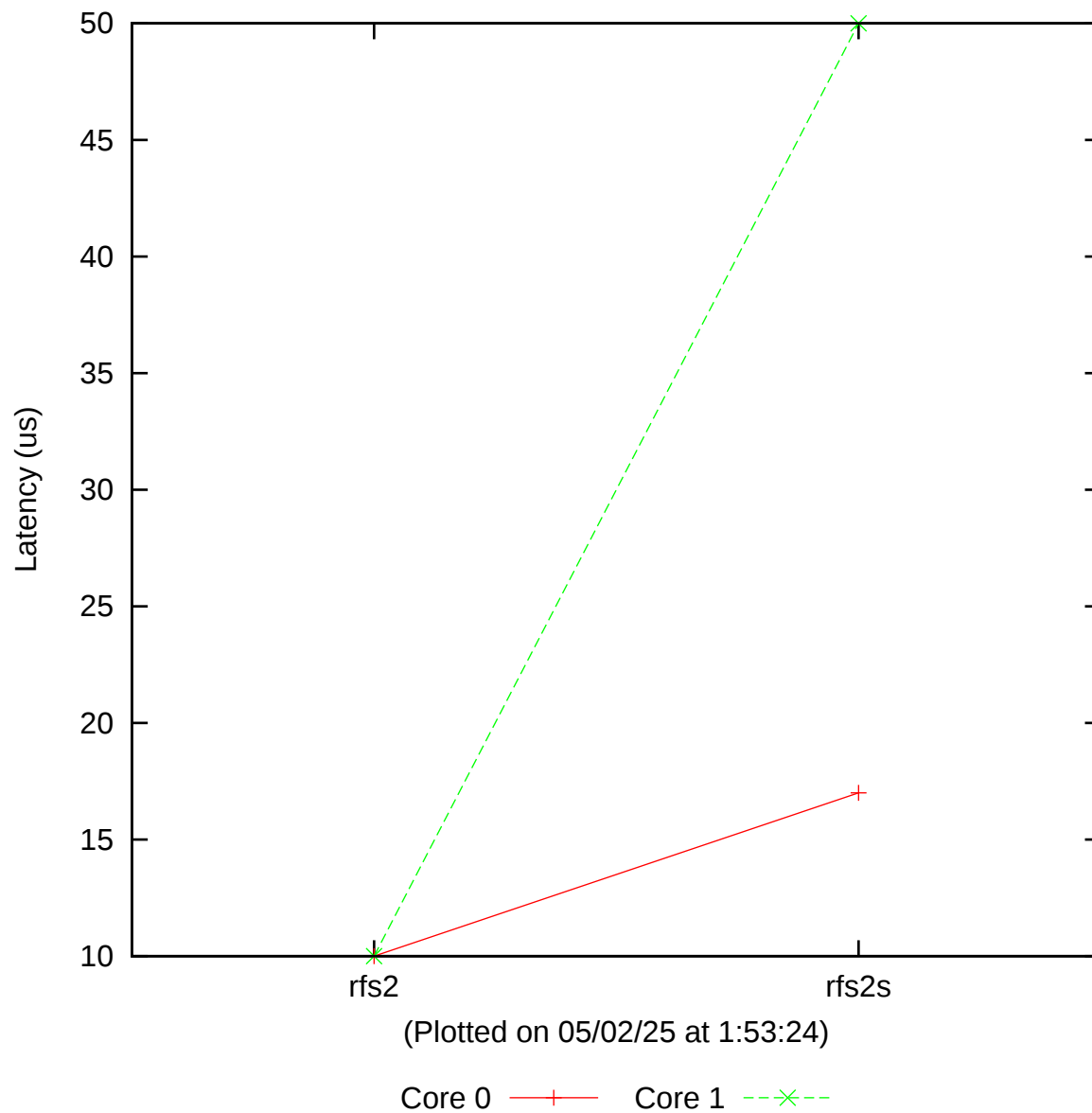
Moderate load maximum latency x86 Intel Core i3-8100H 800 MHz, Linux 5.10.120-rt70-rtss2.4.00.15880 vs. x86 Intel Core i3-8100H 800 MHz, Linux 5.10.120-rt70-rtss2.4.00.15880
